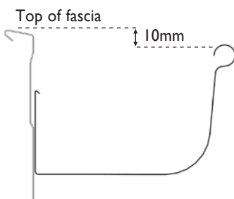
Front of gutter 10mm below top of fascia – overflow capacity 1.5 L/s/m
