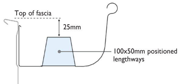
Inverted nozzle at high ends of gutter finished below back of gutter – overflow capacity 1.2L/s
